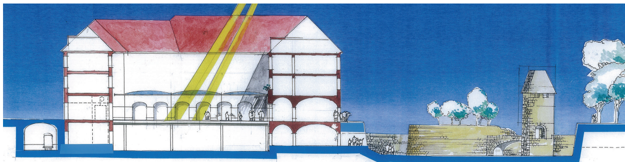
Slika 44: Prerez mahrove hiše z tunelom pod Kopitarjevo ulico in pogled barbakana Picture 44: Cross section through Mah's House with tunnel under Kopitarjeva Street
