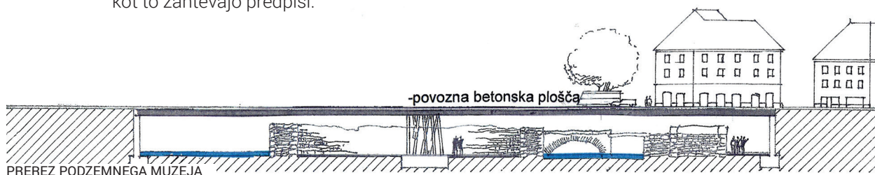
Slika 10: Prerez muzeja 2009 Picture 10: Cross section through subterranean museum, 2009
