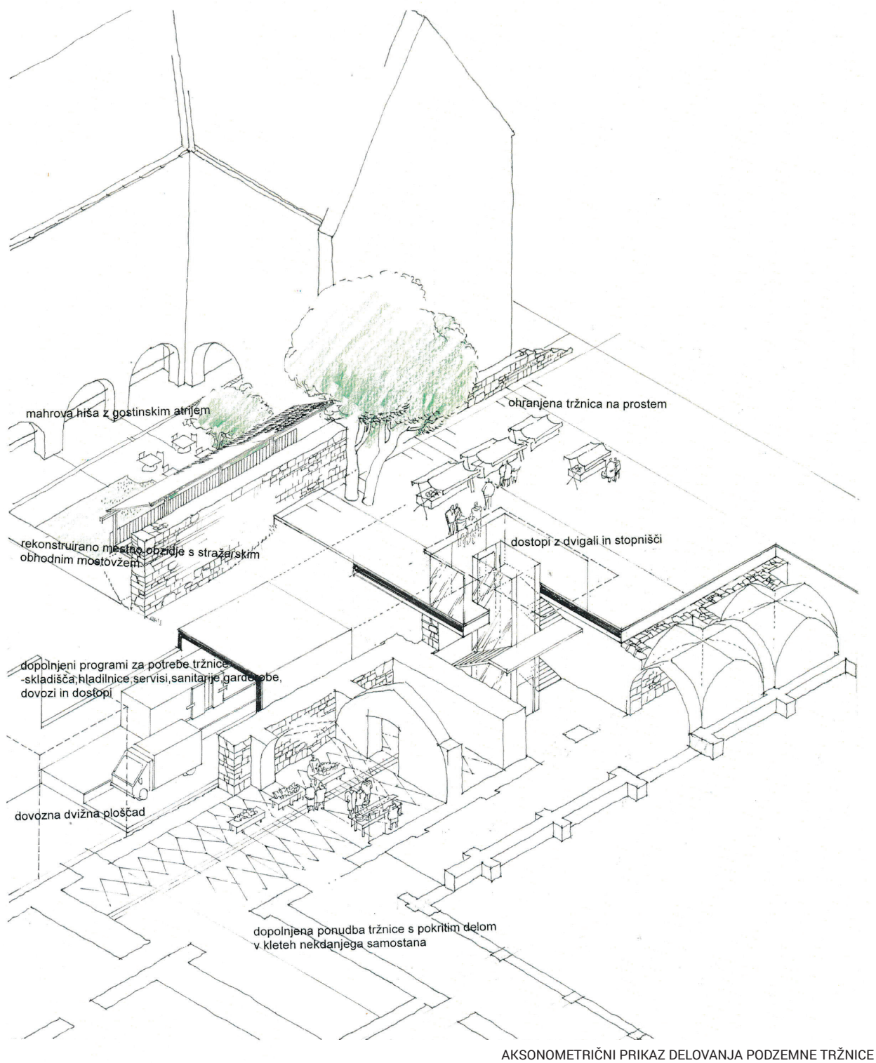
Slika 48: Aksonometrični prerez podzemne tržnice Picture 48: Axiometric section through the subterranean Market place
